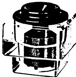
Cut Glass Square Countersunk Inkstands No. 52M No. 52F 3 in. 3 in. Over-all height. 2-1/16 in. 2 3/8 in. Height above desk level. 15/16 in. 5/8 in. Height below desk level. 2 3/4 in. 3 in. Square above desk level. 2-5/16 in. 2 1/4 in. Square below desk level.
